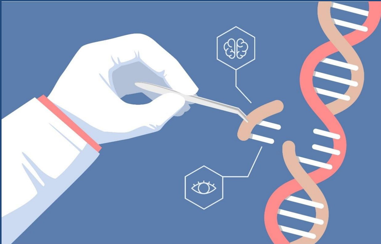
Figure 1 Genomic Editing
