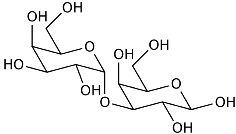
Galactose- \alpha -1,3-galactose (from Wikipedia, public domain)
