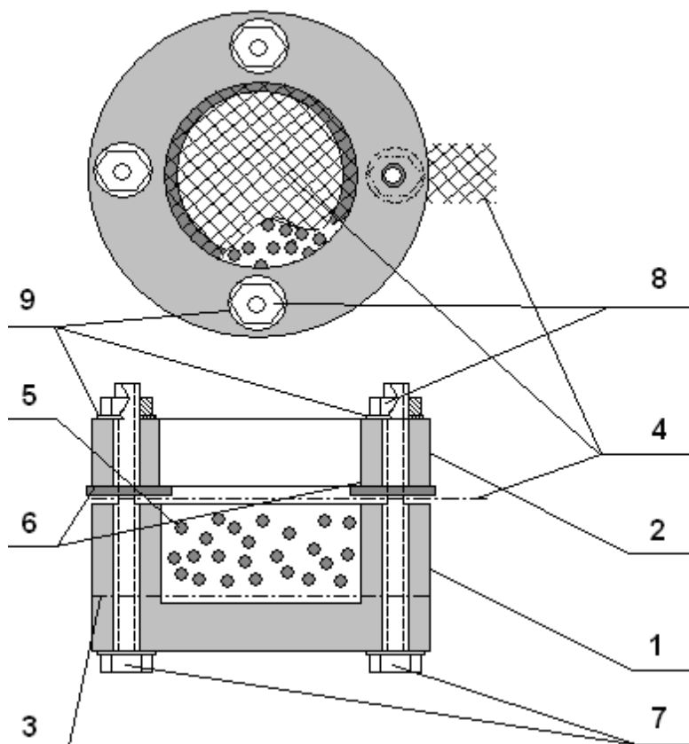
Fig. 1 Column for granulated carbon potential measurements.
