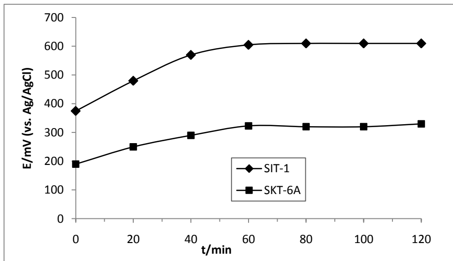
Fig. 2 Open circuit potentials of SIT-1 and SKT-6A vs. time for Medinal adsorption.
